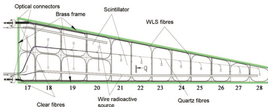
Figure 2. Schematic of the CMS hadron endcap calorimeter scintillator megatiles tiles for tiles in layer 11 through 13. The numbers below the tiles represent the tower number. The megatiles in layers 0 through 4 have an additional tower at large \eta (tower 29). The megatiles in layers 5 through 10 contain tile 16 at low \eta . Layers 14 through 17 do not have tile 17.
