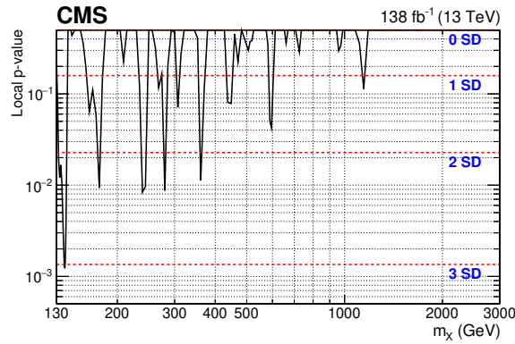
Figure 9. Local p -value as a function of m_X , with f_{\text{VBF}} floating.
