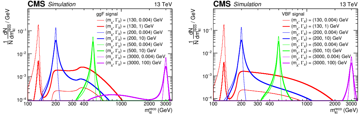
Figure 4. The m_{4\ell}^{\text{reco}} distributions for several values of m_X and \Gamma_X obtained from the signal model, for the ggF (left) and VBF (right) signal processes. All final states and categories are combined.
