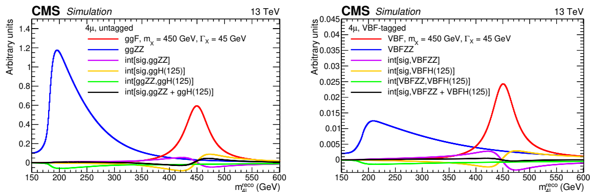
Figure 6. The left (right) plot depicts the lineshapes for the ggF (VBF) signal with m_X = 450 GeV, \Gamma_X = 45 GeV as the red curve, the ggZZ (VBFZZ) background as the blue curve, and interference terms as the violet, orange, and green curves. The black curve shows the interference between the signal and all other SM processes. The notation “int[A,B]” indicates the interference between A and B. Results are shown for the 4\mu final state, for the untagged category (left) and the VBF-tagged category (right).
