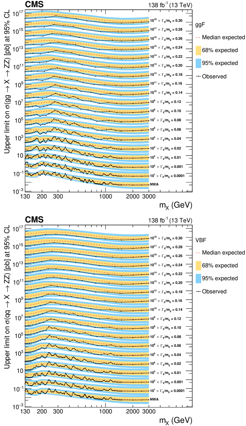
Figure 11. Observed and expected 95% CL upper limits on \sigma(\text{pp} \rightarrow X \rightarrow ZZ) with m_X from 130 GeV to 3 TeV and \Gamma_X/m_X up to 30%. The upper panel shows the results for pure ggF production, and the lower panel shows the results for pure VBF production.
