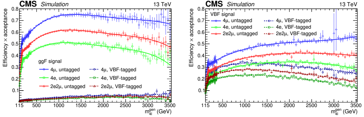
Figure 3. The product of signal efficiency and acceptance, as a function of m_{4\ell}^{\text{gen}} , computed for the 2018 data set. The left panel shows the results for ggF signals, and the right panel shows those for VBF signals. The points are values computed from simulation, which are fitted with the corresponding curves. In each panel, the product of efficiency and acceptance for each final state and category is shown: green squares and curves represent the 4e final state, red rectangles and curves indicate the 2e2 \mu final state, and blue circles and curves the 4 \mu final state; the solid lines with lighter colors represent the untagged category, and the efficiencies for the VBF-tagged categories are shown in dashed lines with darker colors.
