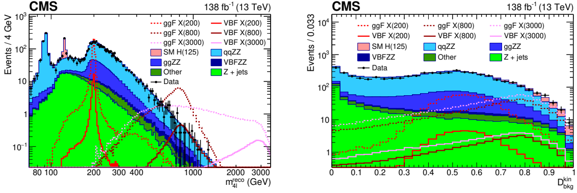
Figure 1. Left: the m_{4\ell}^{reco} distributions for signal and background processes estimated from the MC simulation, alongside observed data. Red and pink open histograms show the lineshapes for different signal masses. Right: the D_{bkg}^{kin} distributions for signal and background processes estimated from the MC simulation, together with the observed data. The masses of the X resonances written in the legends are in GeV units. The widths are 1.43 GeV for m_X = 200 GeV, 304 GeV for m_X = 800 GeV, and 1.5 TeV for m_X = 3 TeV [33].
