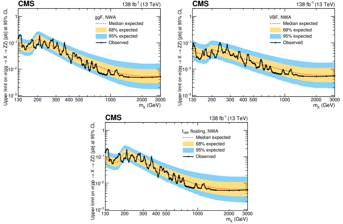
Figure 8. Observed and expected upper limits on \sigma(pp \rightarrow X \rightarrow ZZ) with m_X from 130 GeV to 3 TeV in the narrow-width approximation, for the ggF (upper left) and VBF (upper right) production, and with f_{\text{VBF}} as a free parameter in the fit (lower).
