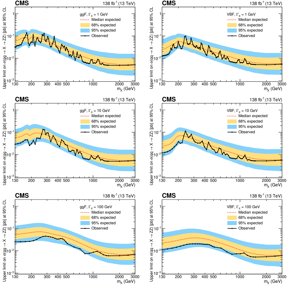
Figure 10. Observed and expected upper limits on \sigma(pp \rightarrow X \rightarrow ZZ) with m_X from 130 GeV to 3 TeV and \Gamma_X equal to 1 (upper), 10 (middle), and 100 (lower) GeV. The left column shows the results for pure ggF production and the right column shows the results for pure VBF production.
