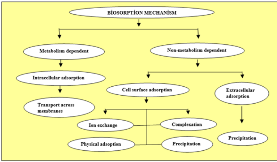
Figure 1. Absorption mechanisms of microorganisms (Güçlü & Ertan, 2011)
