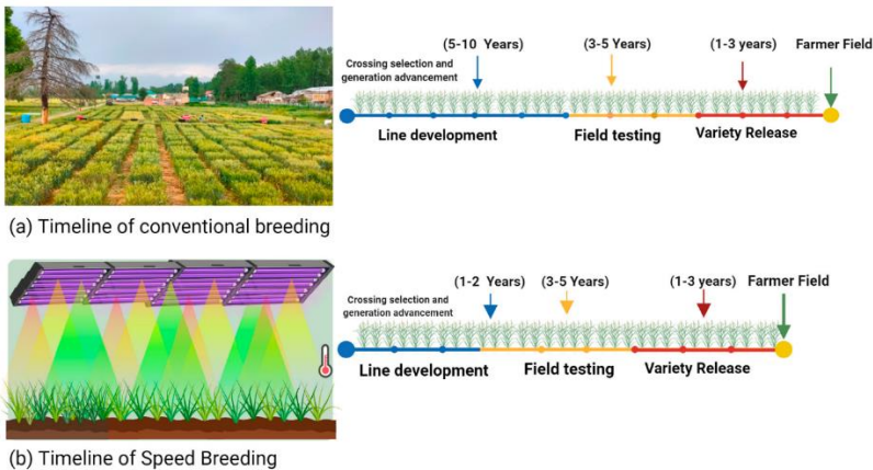
Figure 2. Comparison of traditional breeding and speed breeding (Samantara et. al., 2022).
