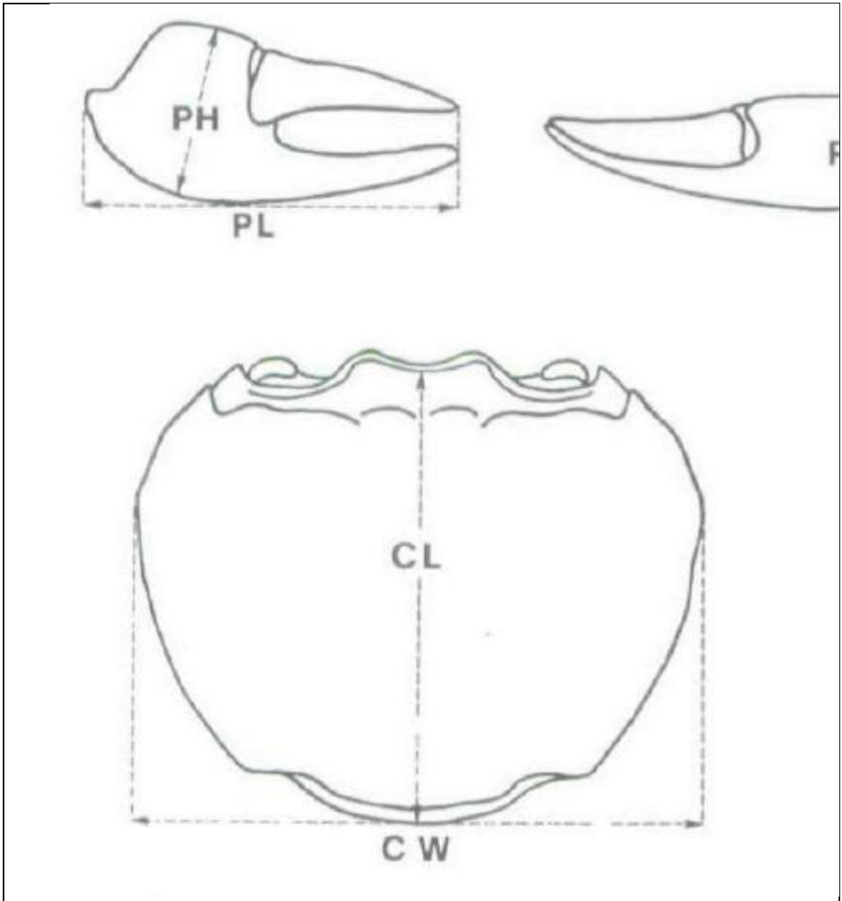
Figure 1. Taking body length parameters in crab (CL, CW, AL, AW, PL, PW, PH) (adapted from Micheli et al., 1990:493)
