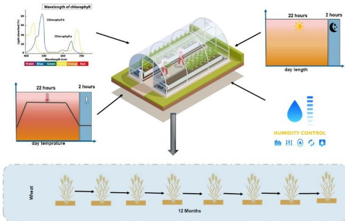
Figure 1. Rapid generation advancement through speed breeding: Experimental crop grown under controlled environments.
