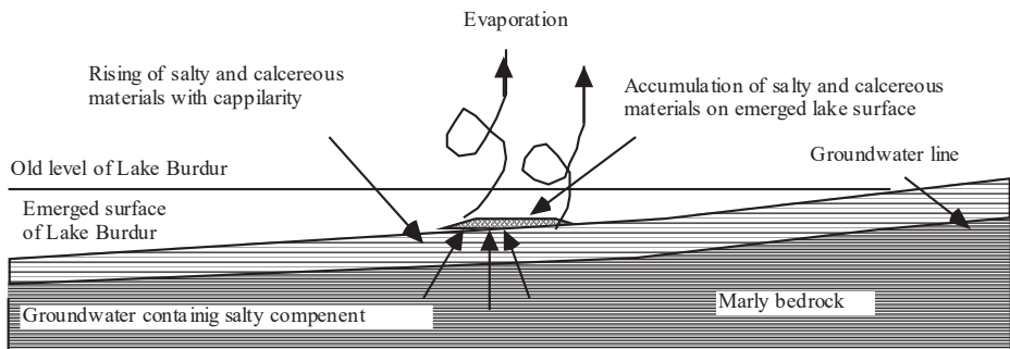
Figure 3. The rising of salty, calcereous material material to be found in the lake water and marly parent material/ bedrock with cappilarity process and the formation of the accumulation of salty and calcereous materials on the emerged Burdur Lake surface (Atalay, et al., 2019)
