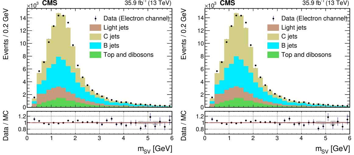
Figure 8. Distribution of the secondary vertex mass m_{SV} of the highest- p_T c-tagged central jet, for electron channel. The observed data is compared to the different signal and background components in simulation, after normalization scale factors as function of Z p_T (left) and c-tagged central jet p_T (right) are applied. Bottom panels on each plot represent the data to MC ratio.
