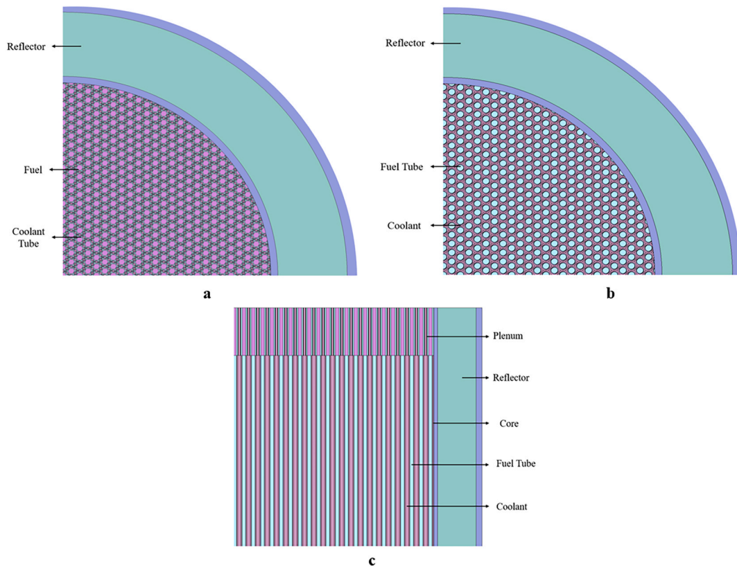
Fig. 3. Serpent model of the DFR m core [10,12].
