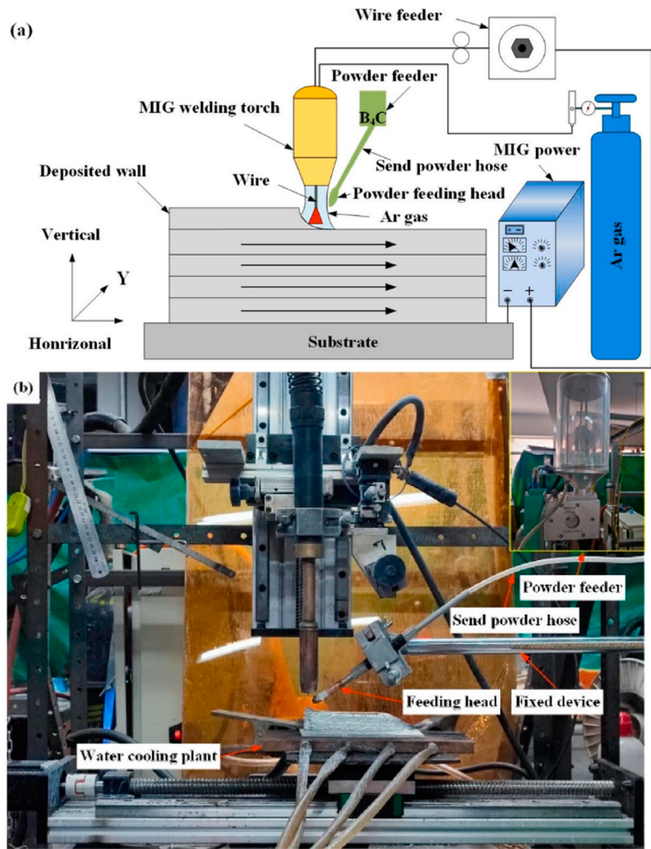
Fig. 16. DP-MIG aluminum alloy powder feeding additive manufacturing (a) Schematic representation of DP-MIG-WAAM aluminum alloy powder feeding manufacturing (b) Demonstration of the experimental equipment of the system [140].
