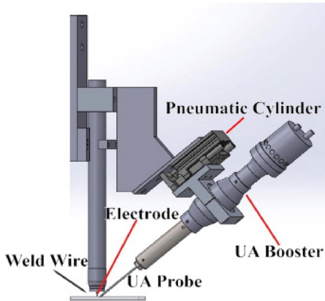
Fig. 15. Illustration of UA-WAAM process [6].
