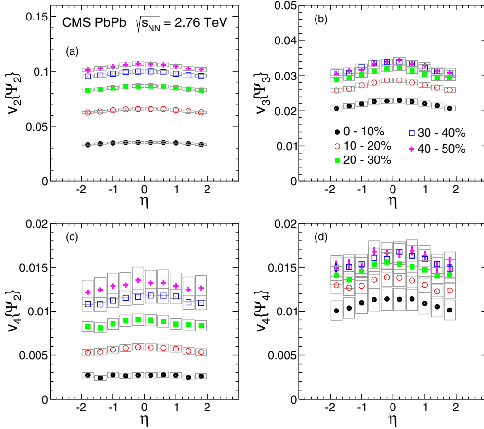
FIG. 8. (Color online) Yield-weighted average azimuthal asymmetry coefficients v_n , for n = 2-4 , with 0.3 < p_T < 3.0 GeV/c are shown as a function of pseudorapidity \eta for the indicated centrality ranges, as specified in percent. Statistical (error bars) and systematic (light gray boxes) uncertainties are shown. The v_2 results are from Ref. [18] and included for completeness.
