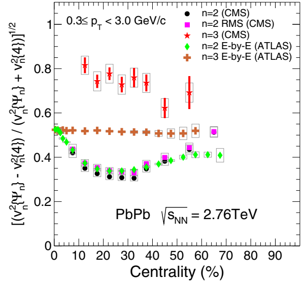
FIG. 15. (Color online) Estimate of the event-by-event v_n fluctuations in v_n for n=2 (solid circles) and n=3 (solid stars) as discussed in the text. The results where the event-plane v_2 values are adjusted to their corresponding rms values, as discussed in the text, are indicated by the solid boxes and labeled n=2 RMS. The results of event-by-event-fluctuation (E-by-E) analyses by the ATLAS Collaboration for the n=2 and 3 harmonics [69] are also shown. Statistical (error bars) and systematic (light gray boxes) uncertainties are indicated. The systematic uncertainties for the ATLAS results correspond to the midpoint of the uncertainty range indicated by the ATLAS Collaboration.
