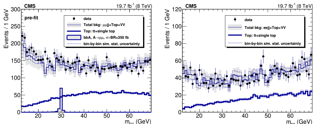
Figure 3. Left: the dimuon mass distribution with the pre-fit expected background event yield and its uncertainty, and the expected signal for m_A = 30 \text{ GeV} assuming a signal cross section times branching fraction of 350 fb. Right: cross-check with the e^+e^- final state showing the dielectron mass spectrum with the expected background event yield and its uncertainty.
