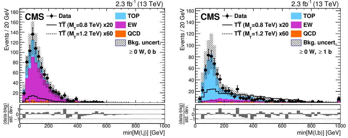
Figure 7. Distributions of \min[M(\ell, j)] in events without b-tagged AK4 jets (left) and \min[M(\ell, b)] in events with \geq 1 b-tagged AK4 jets (right) in the boosted W channel with all categories combined. Also shown are the distributions of T\bar{T} signal events with T quark masses of 0.8 and 1.2 TeV, scaled by factors of 20 and 60, respectively. The uncertainty in the background includes the statistical and systematic uncertainties described in section 7.
