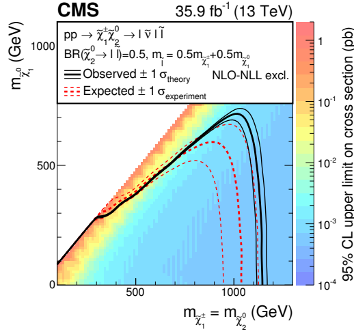
Figure 14. Interpretation of the results in the flavor-democratic model with mass parameter x = 0.5 obtained with events of category A. The shading in the m_{\tilde{\chi}_1^0} versus m_{\tilde{\chi}_1^\pm} (= m_{\tilde{\chi}_2^0}) plane indicates the 95% CL upper limit on the chargino-neutralino production cross section. The contours bound the mass regions excluded at 95% CL assuming the NLO+NLL cross sections. The observed, \pm 1 \sigma_{\text{theory}} ( \pm 1 standard deviation of the theoretical cross section) observed, median expected, and \pm 1 \sigma_{\text{experiment}} expected bounds are shown.
