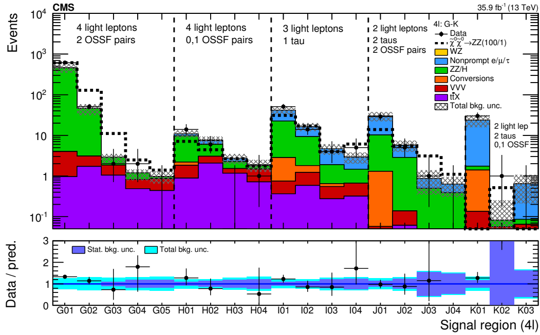
Figure 12. Expected and observed yields comparison in signal regions with at least four leptons (categories G–K). An example mass point in the \tilde{\chi}_1^0 \tilde{\chi}_1^0 production GMSB model is displayed for illustration. The notation is analogous to that used in figure 7.
