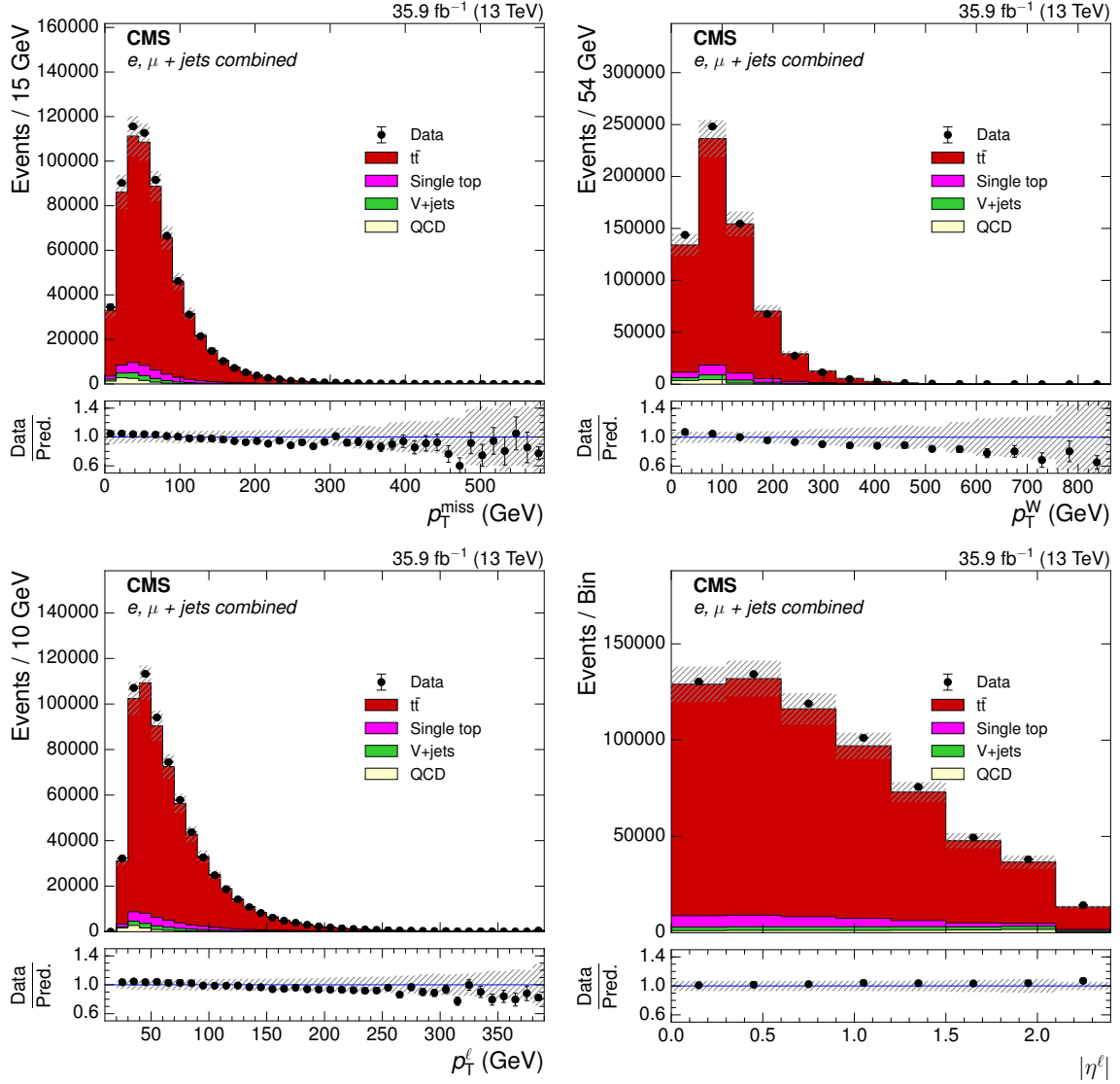
Figure 2. The distributions of p_T^{\text{miss}} , p_T^W , p_T^\ell and |\eta^\ell| after full event selection. The t\bar{t} simulation is normalized to the NNLO prediction. The ratio of the number of events in data to that in simulation is shown below each of the distributions, with the statistical uncertainty in the data shown by the vertical uncertainty bars. The statistical uncertainty in the number of simulation events and the uncertainties in modeling in simulation are shown by the hatched band.
