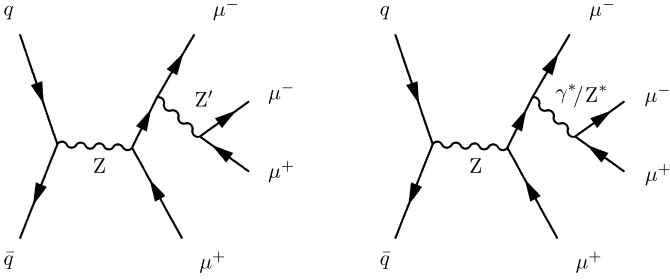
Fig. 1. Leading order Feynman diagrams for the signal process (left) and the dominant background process (right), where in each diagram the four-muon final state originates from annihilation.
