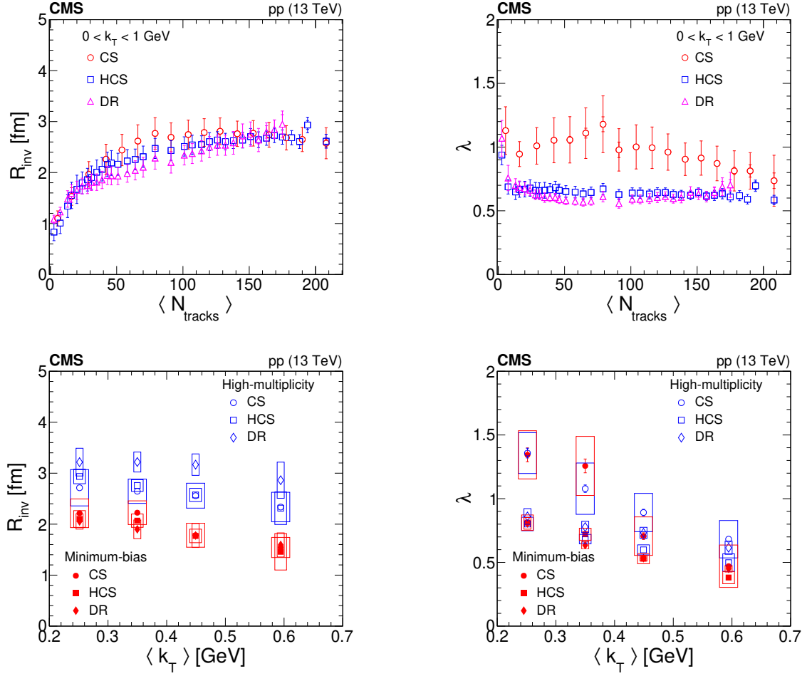
Figure 4. Results for R_{\text{inv}} (left) and \lambda (right) from the three methods as a function of multiplicity (upper) and k_T (lower). In the upper plots, statistical and systematic uncertainties are represented by internal and external error bars, respectively. In the lower plots, statistical and systematic uncertainties are shown as error bars and open boxes, respectively.
