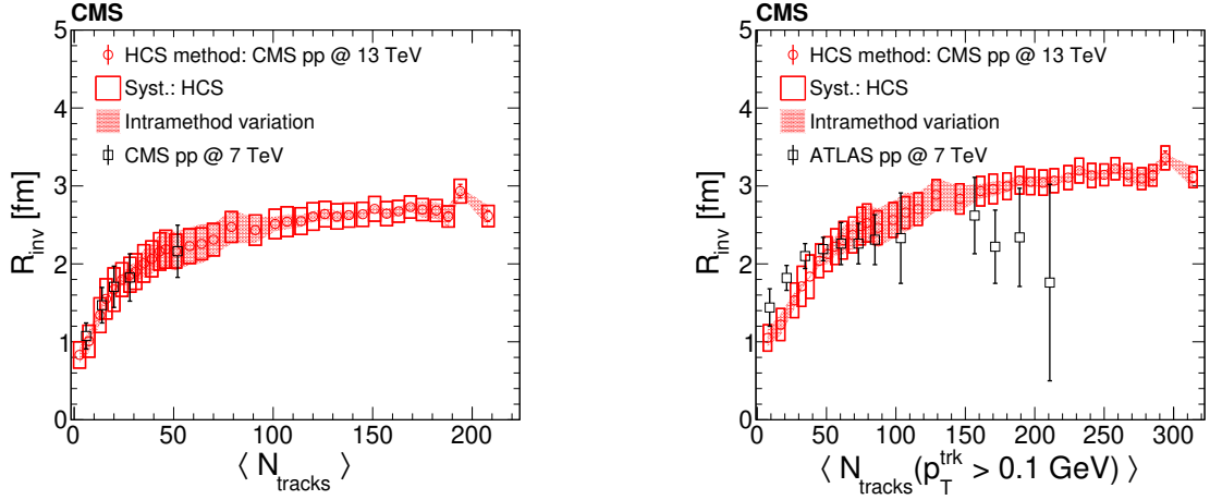
Figure 5. The R_{\text{inv}} fit parameters as a function of particle-level multiplicities using the HCS method in pp collisions at 13 TeV compared to results for pp collisions at 7 TeV from CMS (left) and ATLAS (right). Both the ordinate and abscissa for the CMS data in the right plot have been adjusted for compatibility with the ATLAS analysis procedure, as explained in the text. The error bars in the CMS [5] case represent systematic uncertainties (statistical uncertainties are smaller than the marker size) and in the ATLAS [15] case, statistical and systematic uncertainties added in quadrature.
