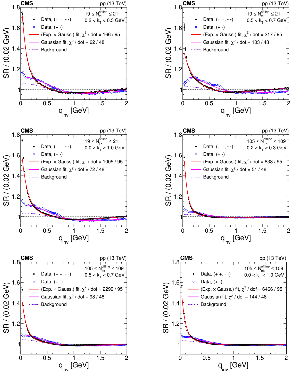
Figure 3. The same-sign (+, +, - -) and opposite-sign (+, -) single ratios in data for different bins of N_{trk}^{offline} and k_T , with their respective fits. The label “(Exp. \times Gauss.) fit” refers to the same-sign data and is given by eq. (5.7). The label “Gaussian fit” corresponds to eq. (5.4) applied to opposite-sign data and “Background” is the component of eq. (5.7) that is found from the Gaussian fit using eqs. (5.5) and (5.6) to convert the fit parameters. Coulomb corrections are accounted for using the Gamow factor. The error bars represent statistical uncertainties and in most cases are smaller than the marker size.
