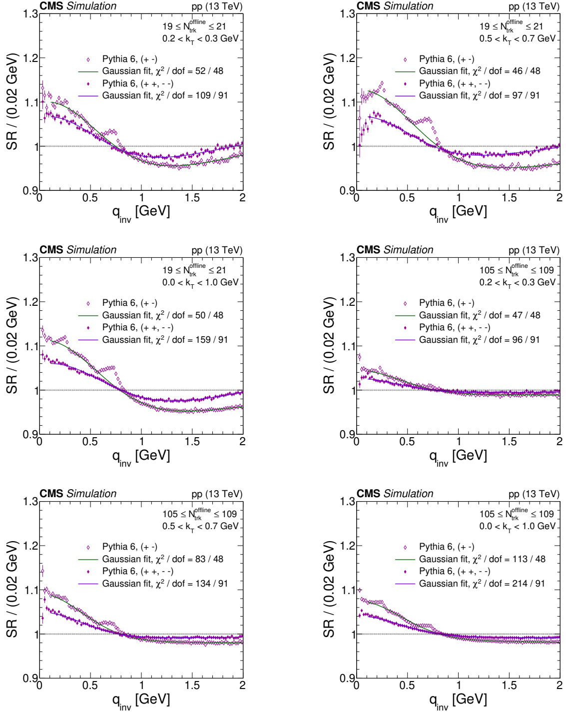
Figure 1. The same-sign ( ++ , -- ) and opposite-sign ( +- ) single ratios employing PYTHIA 6 (Z2* tune) in different bins of N_{\text{trk}}^{\text{offline}} and k_T with the respective Gaussian fit from eq. (5.4). The following q_{\text{inv}} ranges are excluded from the fits to the opposite sign single ratios: 0.2 < q_{\text{inv}} < 0.3 , 0.4 < q_{\text{inv}} < 0.9 , and 0.95 < q_{\text{inv}} < 1.2 GeV. Coulomb interactions are not included in the simulation. The error bars represent statistical uncertainties and in most cases are smaller than the marker size.
