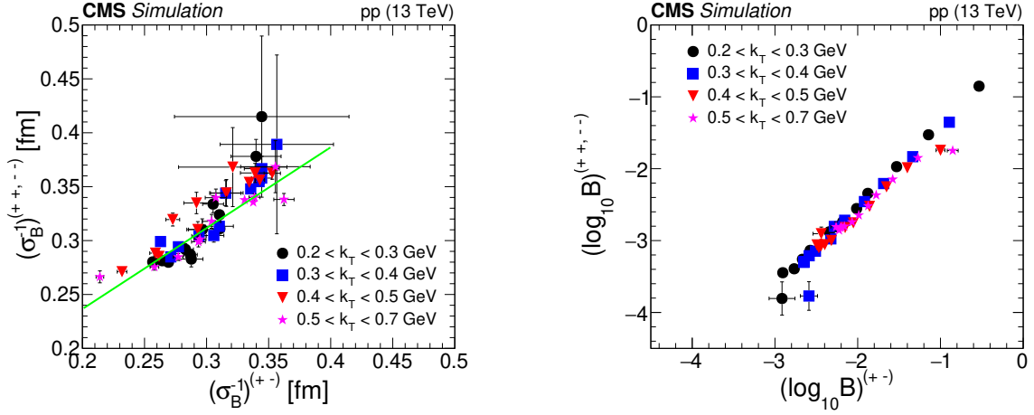
Figure 2. Relations between same-sign (++, --) and opposite-sign (+-) fit parameters from eq. (5.4), as a function of k_T and N_{\text{trk}}^{\text{offline}} for events in MB (i.e., higher \sigma_B^{-1} and lower \log_{10} B ) and HM (i.e., lower \sigma_B^{-1} and higher \log_{10} B ) ranges. The fit values found for the parameters corresponding to the peak's width (left) and the amplitude (right) of the same-sign and opposite-sign correlations are shown. For a given k_T range, each point represents an N_{\text{trk}}^{\text{offline}} bin. The line in the left plot is a linear fit to all the data. The error bars represent statistical uncertainties.
