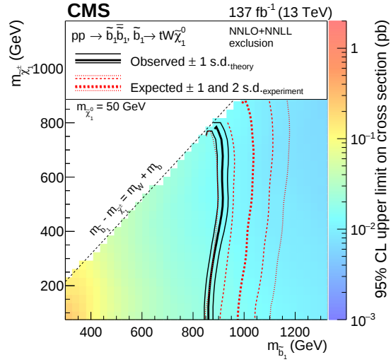
Figure 10: Exclusion regions at 95% CL in the plane of m_{\tilde{\chi}_1^\pm} versus m_{\tilde{b}_1} for the T6ttWW model with m_{\tilde{\chi}_1^0} = 50 GeV. The notations are as in Fig. 7.
