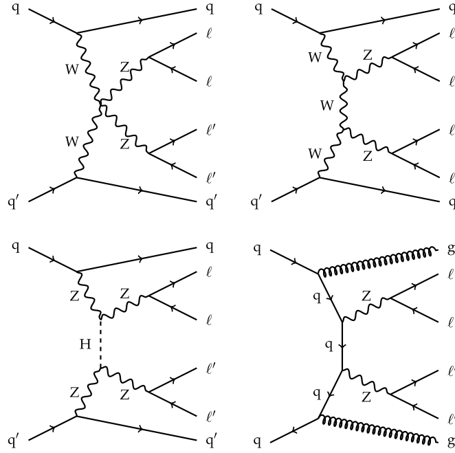
Fig. 1. Representative Feynman diagrams for the EW- (top row and bottom left) and QCD-induced (bottom right) production of the ZZjj \rightarrow \ell\ell\ell'\ell'jj ( \ell, \ell' = e, \mu ) final state. The scattering of massive gauge bosons as depicted in the top row is unitarized by the interference with amplitudes that feature the Higgs boson (bottom left).
