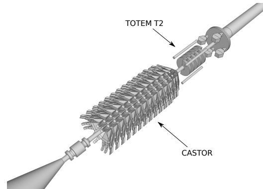
Figure 2. Left: closeup image of the CASTOR calorimeter surrounded by the CMS collar shielding in the open position during an integration test, about 5 m below the beam pipe. Right: visualization of the CASTOR detector integrated around the beam pipe. The CMS interaction point is at 14.4 m upstream (towards the upper right). The TOTEM T2 tracking station, and several pieces of LHC/CMS infrastructure, are visible along this direction.
