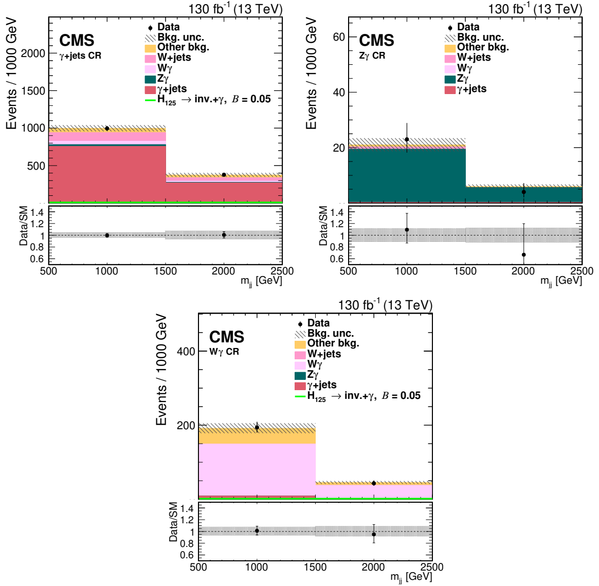
Figure 2. The m_{jj} distributions from the simultaneous fit in the \gamma + \text{jets} (upper left), Z(\mu^+\mu^-) + \gamma (upper right), and W(\mu\nu) + \gamma (lower) CRs. The category other background includes contributions from Z + \text{jets} , nonprompt, top quark, VV , and VVV processes. Overflow events are included in the last bin. The shaded bands represent the combination of the statistical and systematic uncertainties in the predicted yields. The light green line, illustrating the possible contribution expected from inclusive SM Higgs boson production, assumes a branching fraction of 5% for H \rightarrow \text{inv.} + \gamma decays. The lower panel in the figures shows a per-bin ratio of the data yield and the background expectation. The shaded band corresponds to the combined systematic and statistical uncertainty in the background expectation.
