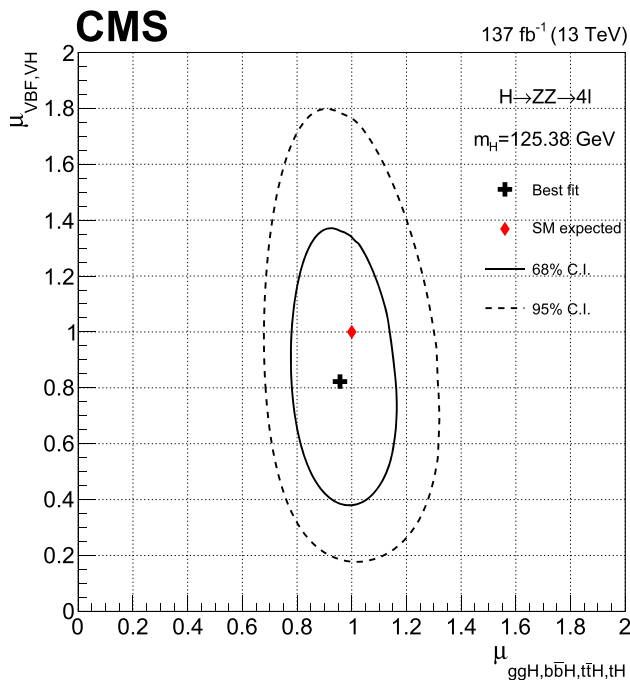
Fig. 12 Result of the 2D likelihood scan for the \mu_f \equiv \mu_{ggH, t\bar{t}H, b\bar{b}H, tH} and \mu_V \equiv \mu_{VBF, VH} signal strength modifiers. The solid and dashed contours show the 68 and 95% CL regions, respectively. The cross indicates the best fit value, and the diamond represents the expected value for the SM Higgs boson
