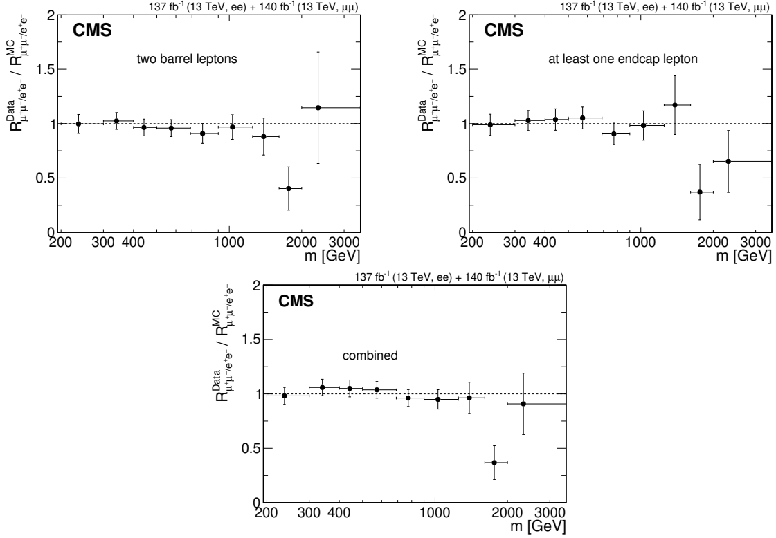
Figure 12. Ratio of the differential dilepton production cross section in the dimuon and dielectron channels R_{\mu\mu/e e}^{Data}/R_{\mu\mu/e e}^{MC} , as a function of m_{\ell\ell} for (upper left) events with two barrel leptons, (upper right) at least one lepton in the endcaps, and (lower) their combination. The ratio is obtained after correcting the reconstructed mass spectra to particle level. The error bars include both statistical and systematic uncertainties.
