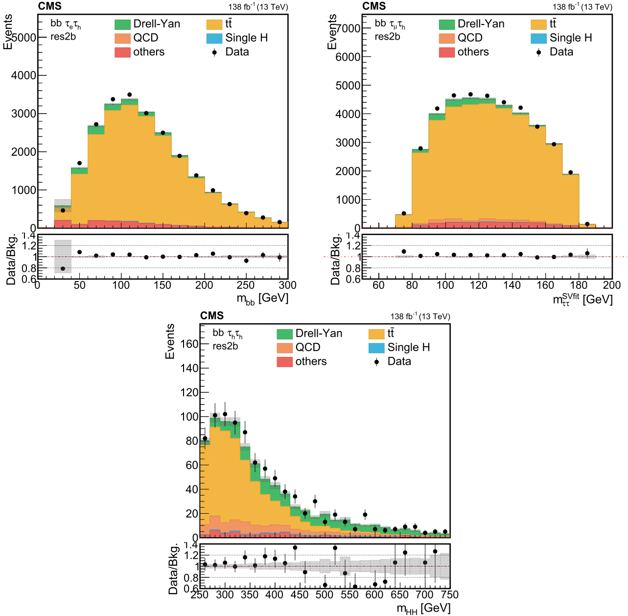
Fig. 3. Distributions of the reconstructed mass of the bb (upper left), \tau\tau (upper right) and HH (lower) pairs in the most sensitive category of the analysis ( res2b ). Events are shown in the \tau_e\tau_h (upper left), \tau_\mu\tau_h (upper right) and \tau_h\tau_h (lower) channels for the full 2016–2018 data set, after the selection on the reconstructed masses of the \tau\tau and bb pairs, as described in Section 5. The shaded band in the plots represents the statistical uncertainty only.
