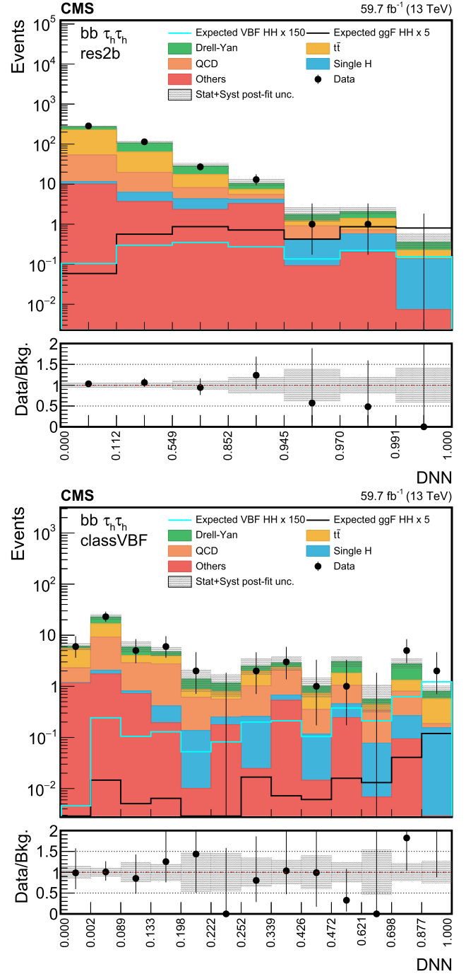
Fig. 4. The postfit DNN distributions in the \tau_h \tau_h channel in 2018 for the most sensitive category in the ggF (upper) and VBF (lower) searches. The shaded band in the plots represents the statistical plus systematic uncertainty. The expected SM distributions for the ggF and VBF HH signals are shown superimposed on the figures.
