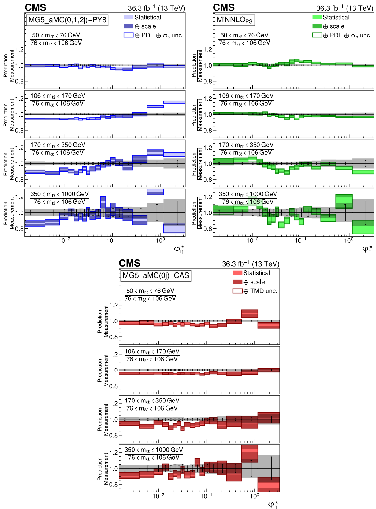
Fig. 23 Ratios of differential cross sections in \phi_{\ell\ell}^* for invariant m_{\ell\ell} with respect to the peak region 76 < m_{\ell\ell} < 106 GeV. Compared to model predictions from MG5_aMC (0, 1, and 2 jets at NLO) + PYTHIA
