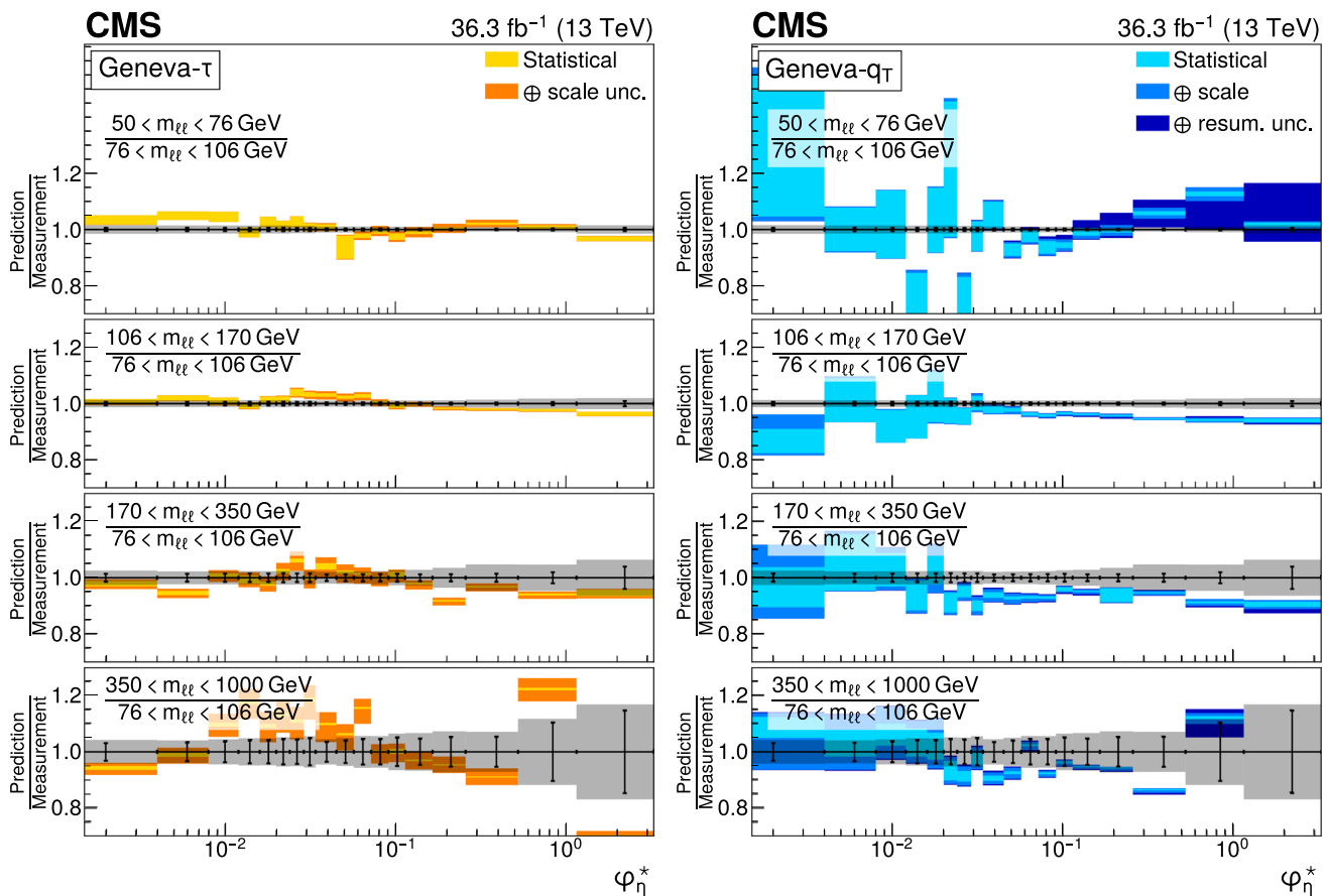
Fig. 24 Ratios of differential cross sections in \varphi_n^*(\ell\ell) for invariant m_{\ell\ell} with respect to the peak region 76 < m_{\ell\ell} < 106 GeV. Compared to model predictions from GENEVA- \tau (left) and GENEVA- q_T (right). Details on the presentation of the results are given in Fig. 8 caption
