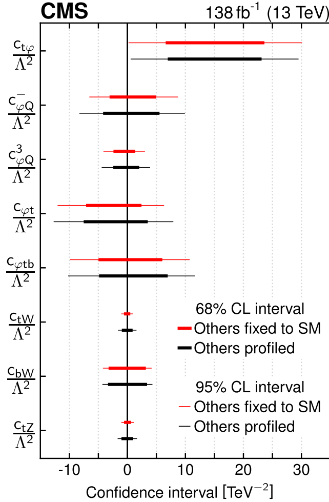
FIG. 10. The observed 68% and 95% CL intervals for the WCs are shown by the thick and thin bars, respectively. The intervals are found by scanning over a single WC while either profiling the other seven WCs (black) or fixing them to the SM value of zero (red).
