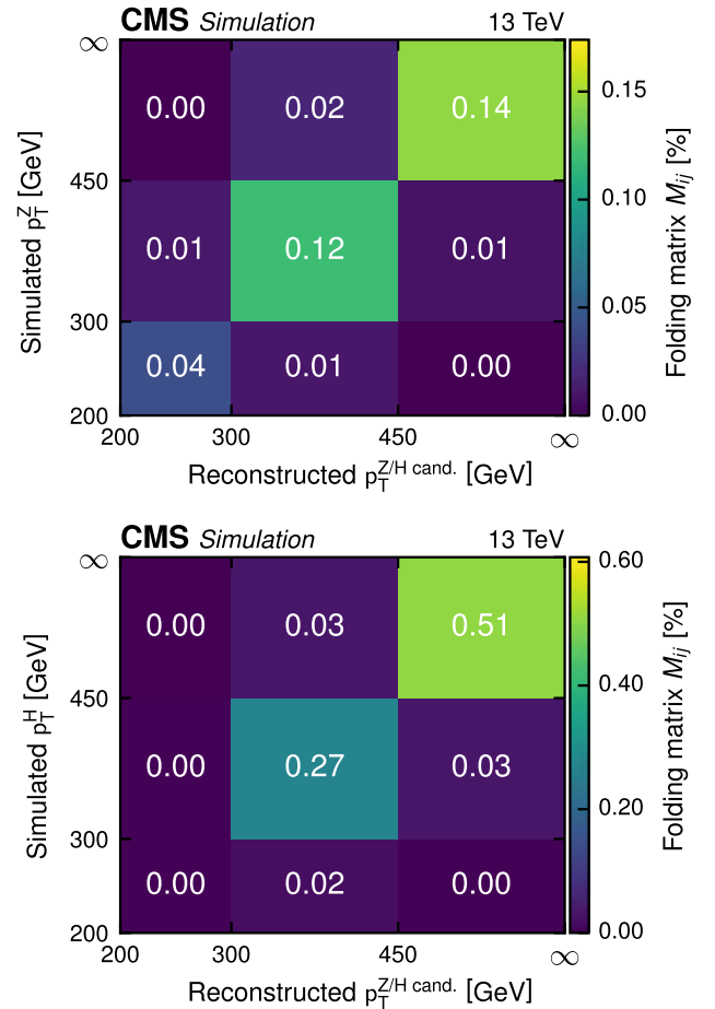
FIG. 5. The percentage of simulated \bar{t}tZ (upper) and \bar{t}tH (lower) signal events that satisfy the baseline event selection requirements as well as the DNN and mass requirements in bins defined by the reconstructed AK8 jet p_T (x axis) and simulated p_T^{Z/H} (y axis). The rightmost and uppermost bins are unbounded. The value of each bin is the ratio of the event yield in the bin to the total number of simulated signal events with a simulated p_T^{Z/H} in the same y-axis bin, including all decay modes of the top quark, Z boson, and Higgs boson. The color scale to the right shows the meaning of the histogram colors.
