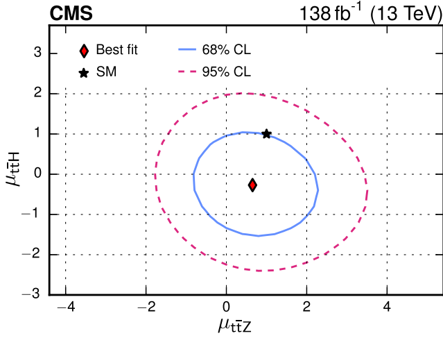
FIG. 7. The observed best fit values (diamond) and SM predictions (star) for the signal strength modifiers \mu_{tH} versus \mu_{tZ} for generator-level p_T^H or p_T^Z > 200 GeV. The solid blue and dashed red contours show the 68% and 95% CL regions, respectively.
