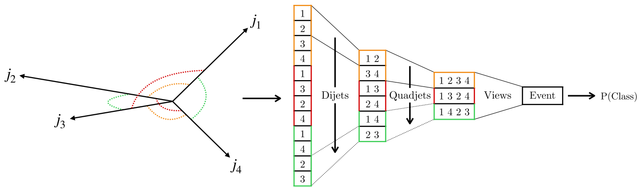
Fig. 3 A high-level sketch of the HCR classifier architecture. Boson-candidate jets are shown on the left with the three possible jet pairings. The HCR architecture is shown on the right. The boxes represent pixels, with the labels indicating which jet, dijet, or quadjet the pixel refers to.
