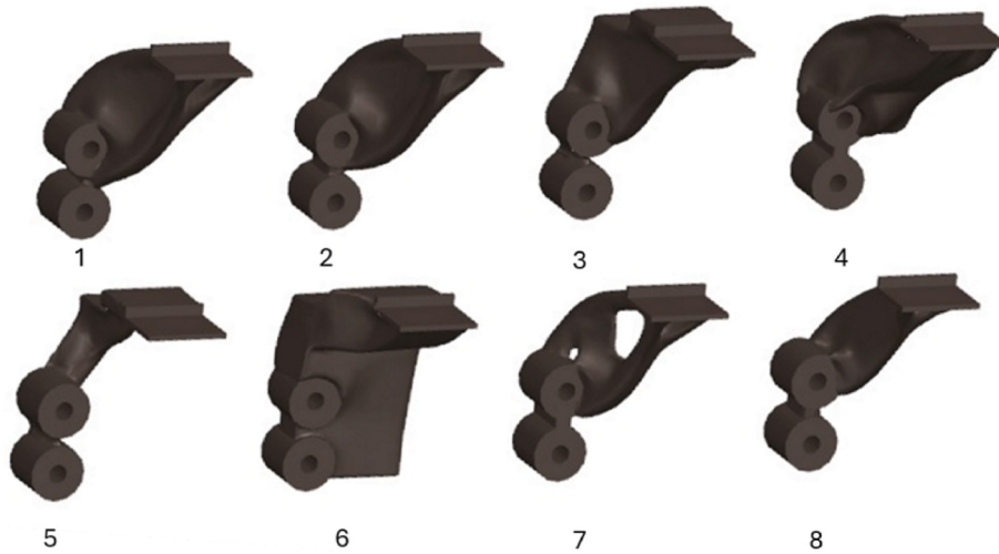
Fig. 19. Redesigned alternative geometries.
