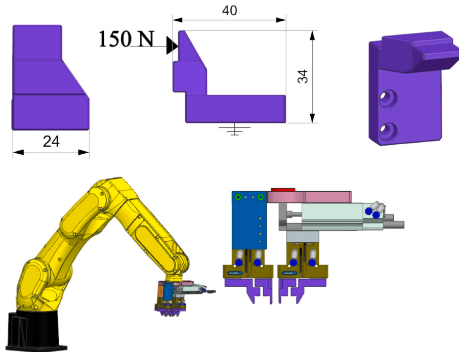
Fig. 17. Available gripper model and its dimensions.
